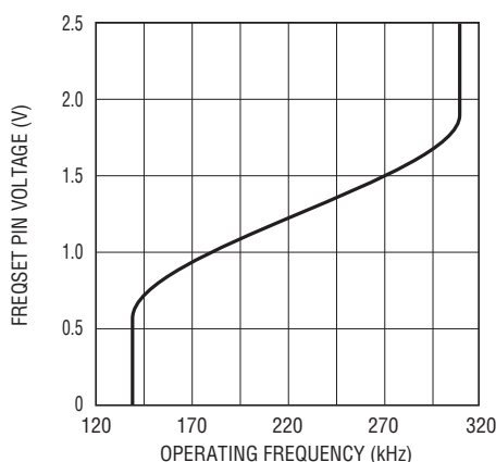
Figure 5. FREQSET Pin Voltage vs Frequency
