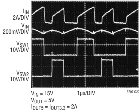
Input Source/Capacitor Instantaneous Current (Figure 13)
